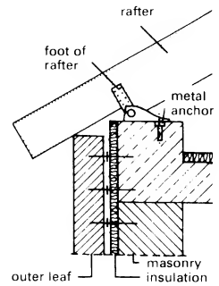
6 Steel rafter connection
